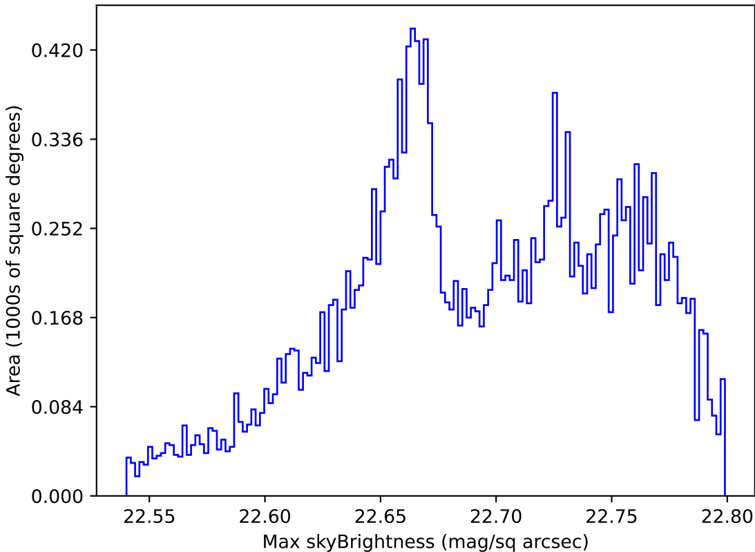
too_5_4v3.4_10yrs All sky u band: Max skyBrightness
