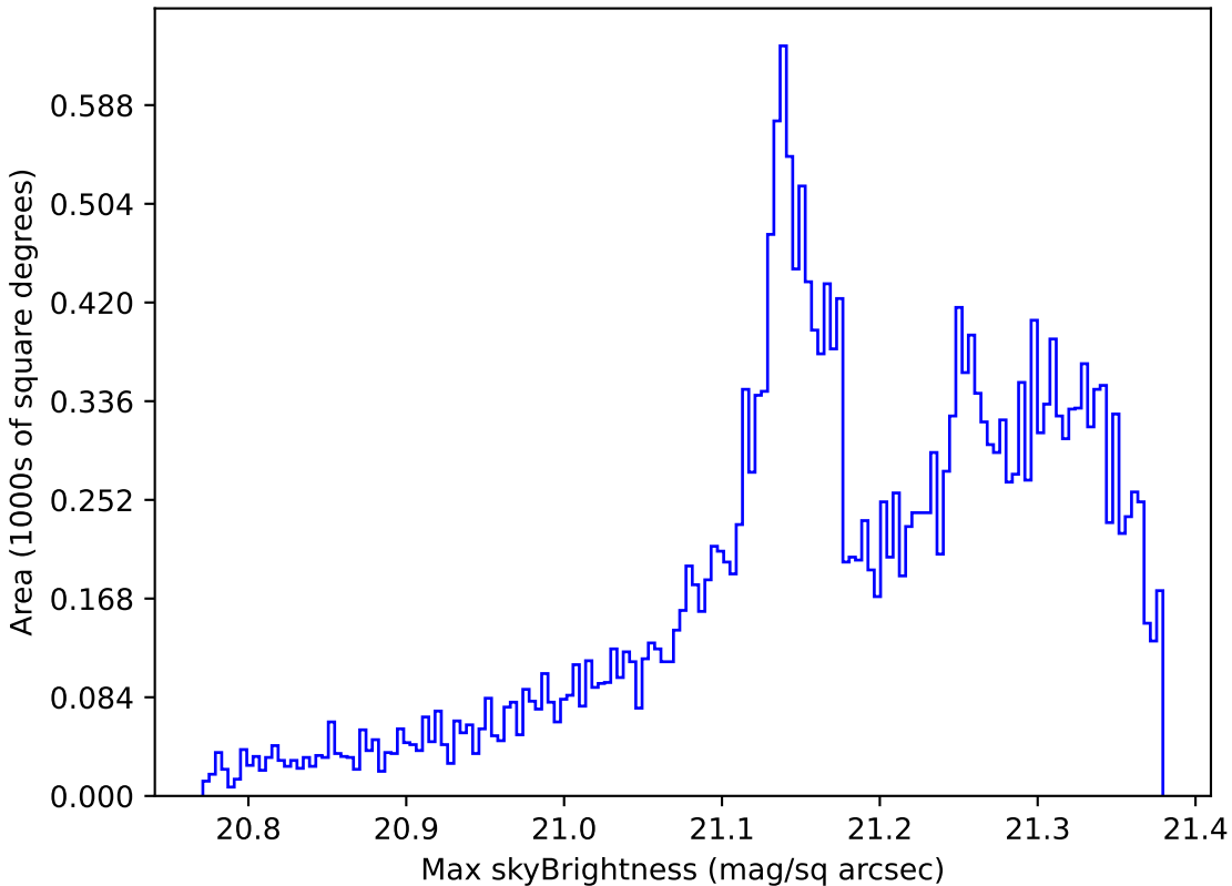
too_5_4v3.4_10yrs All sky r band: Max skyBrightness
