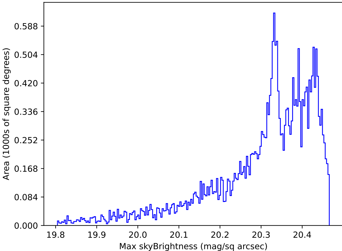
too_5_4v3.4_10yrs All sky i band: Max skyBrightness
