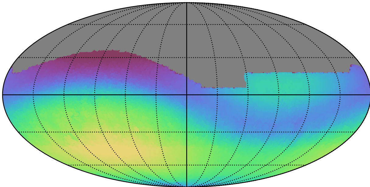
too_5_4v3.4_10yrs All sky g band: Max skyBrightness
