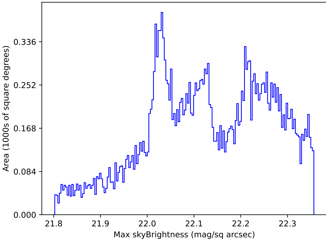
too_5_4v3.4_10yrs All sky g band: Max skyBrightness
