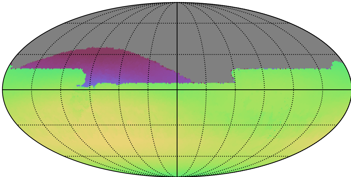
too_5_4v3.4_10yrs All sky all bands: Max skyBrightness
