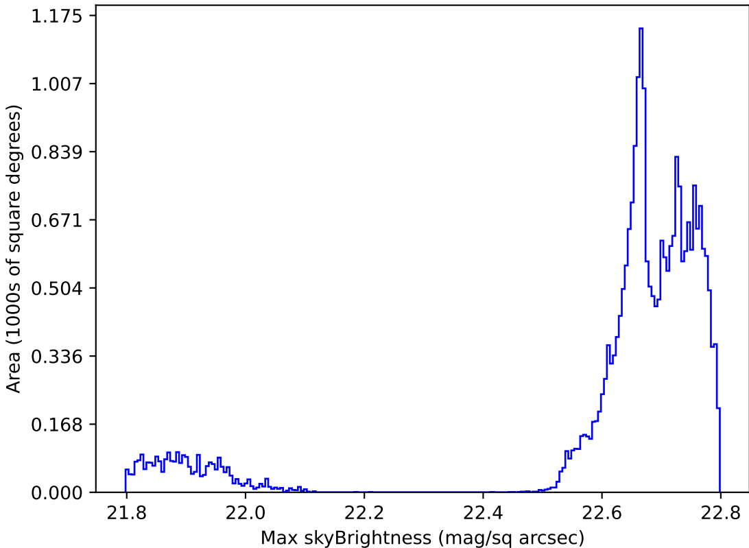
too_5_4v3.4_10yrs All sky all bands: Max skyBrightness
