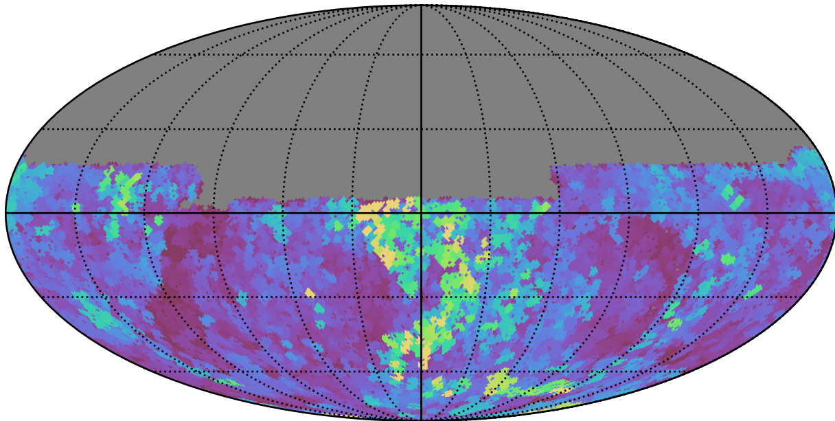
too_5_4v3.4_10yrs Yr 1 y band: Max seeingGeom
