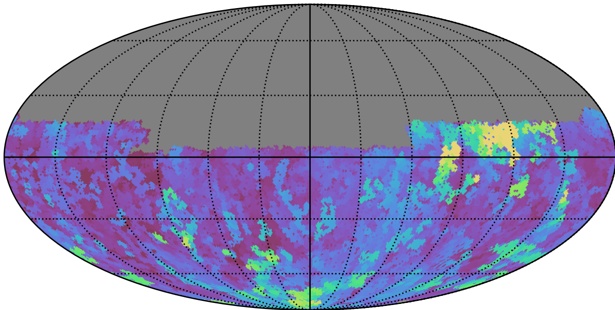
too_5_4v3.4_10yrs Yr 1 u band: Max seeingGeom
