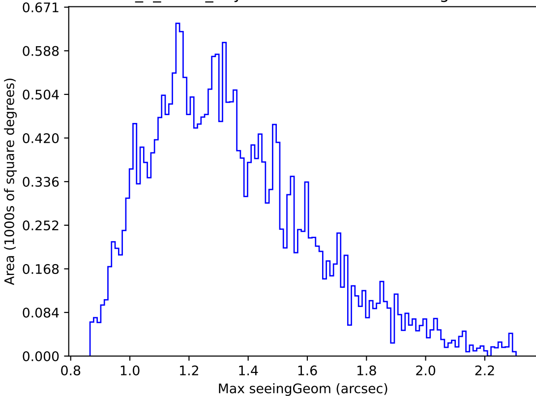
too_5_4v3.4_10yrs Yr 1 r band: Max seeingGeom
