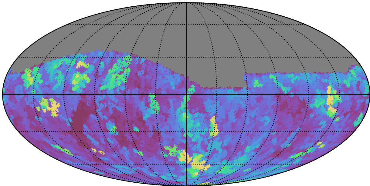
too_5_4v3.4_10yrs Yr 1 i band: Max seeingGeom
