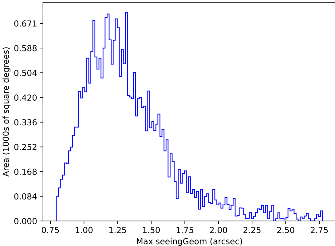
too_5_4v3.4_10yrs Yr 1 g band: Max seeingGeom
