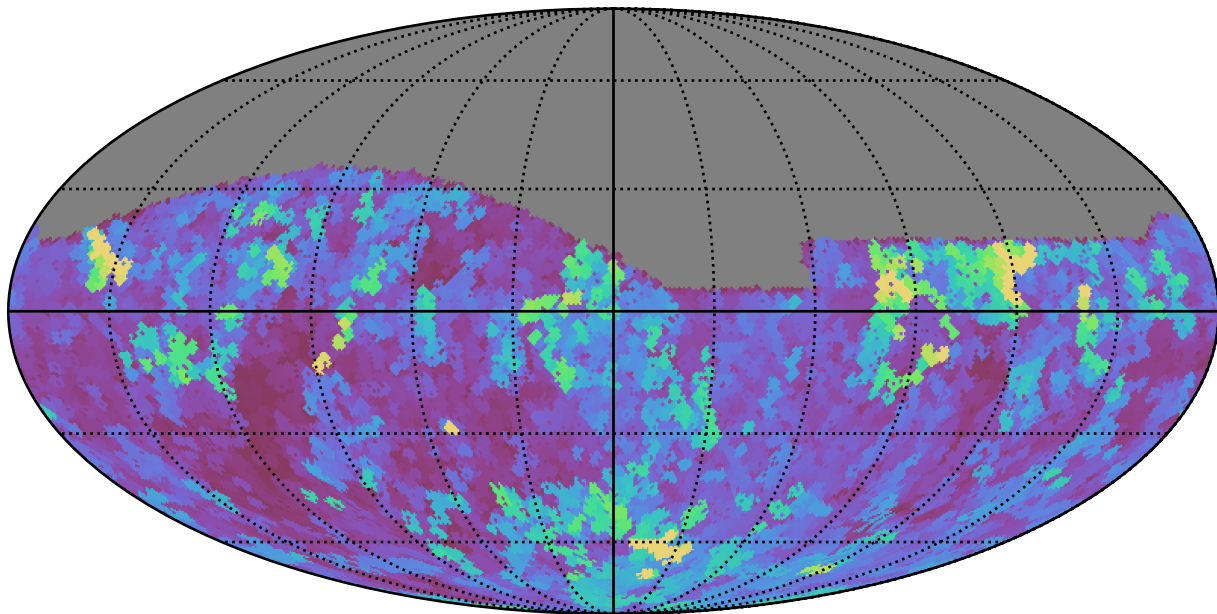
too_5_4v3.4_10yrs Yr 1 all bands: Max seeingGeom
