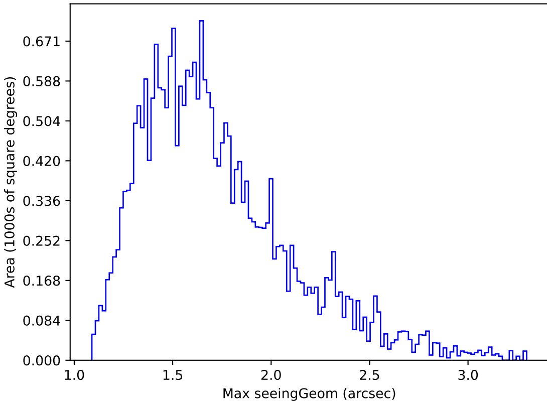
too_5_4v3.4_10yrs Yr 1 all bands: Max seeingGeom
