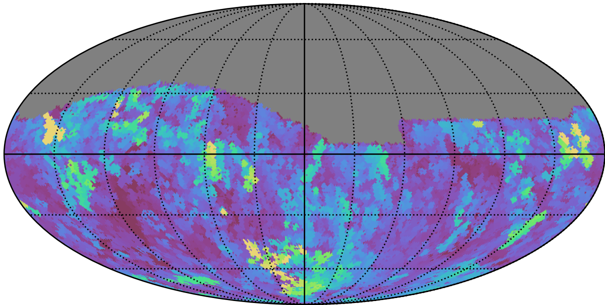
too_5_4v3.4_10yrs Yr 1 z band: Max seeingEff
