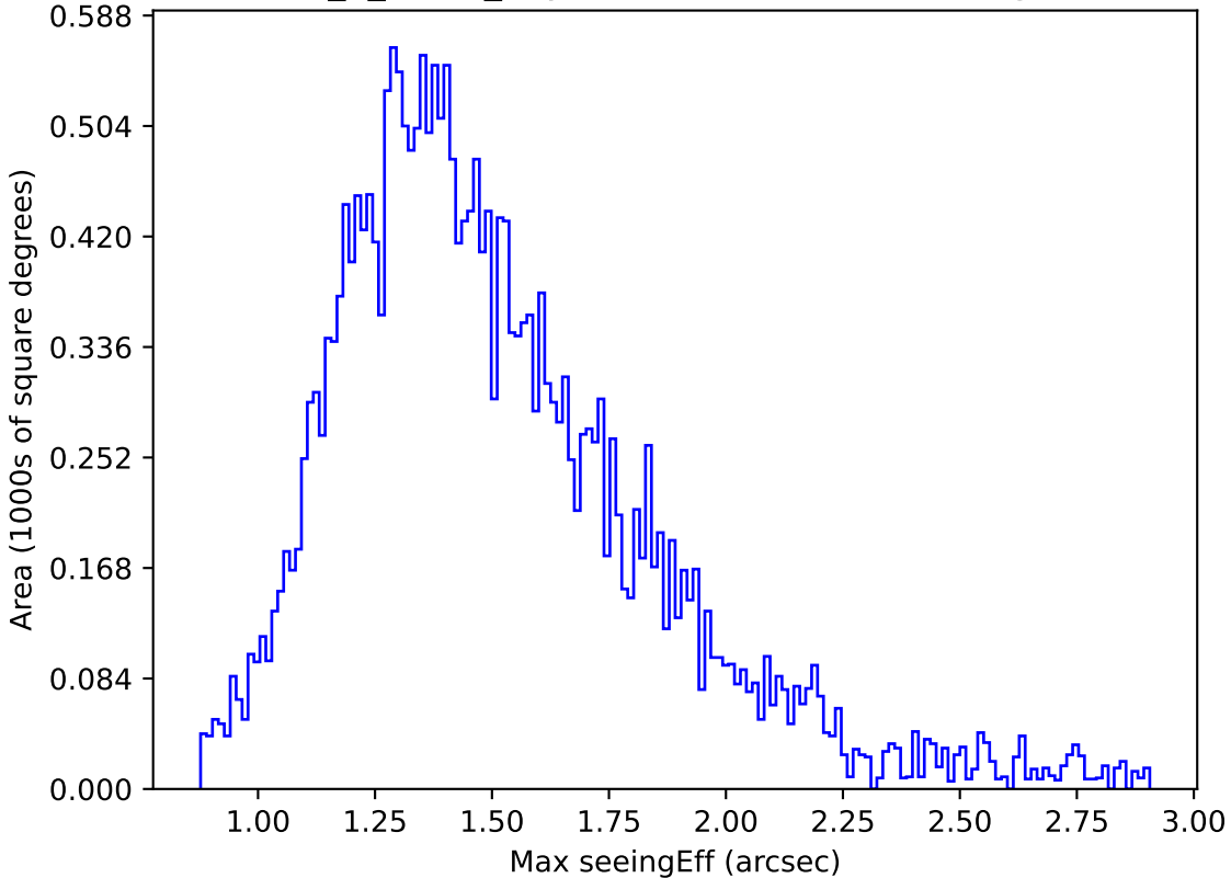
too_5_4v3.4_10yrs Yr 1 z band: Max seeingEff
