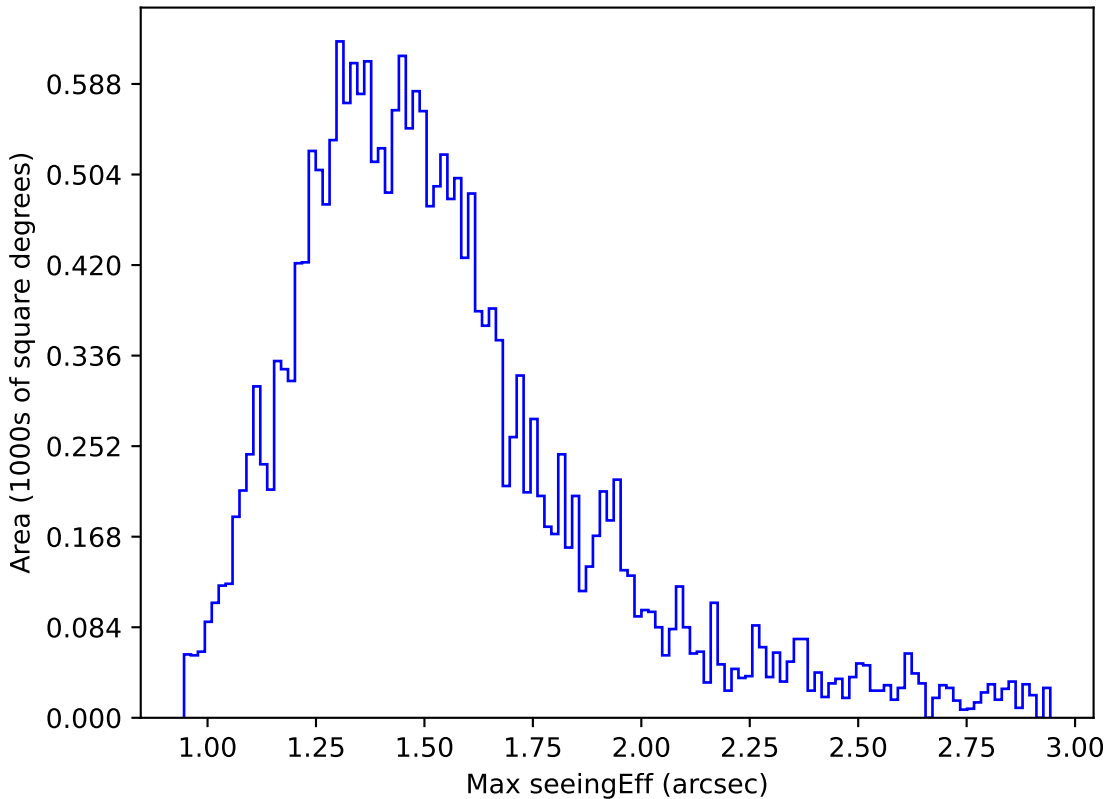
too_5_4v3.4_10yrs Yr 1 y band: Max seeingEff
