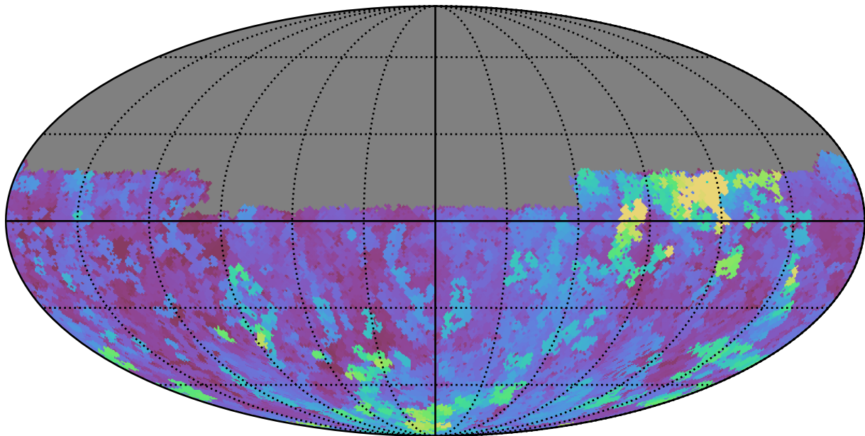
too_5_4v3.4_10yrs Yr 1 u band: Max seeingEff
