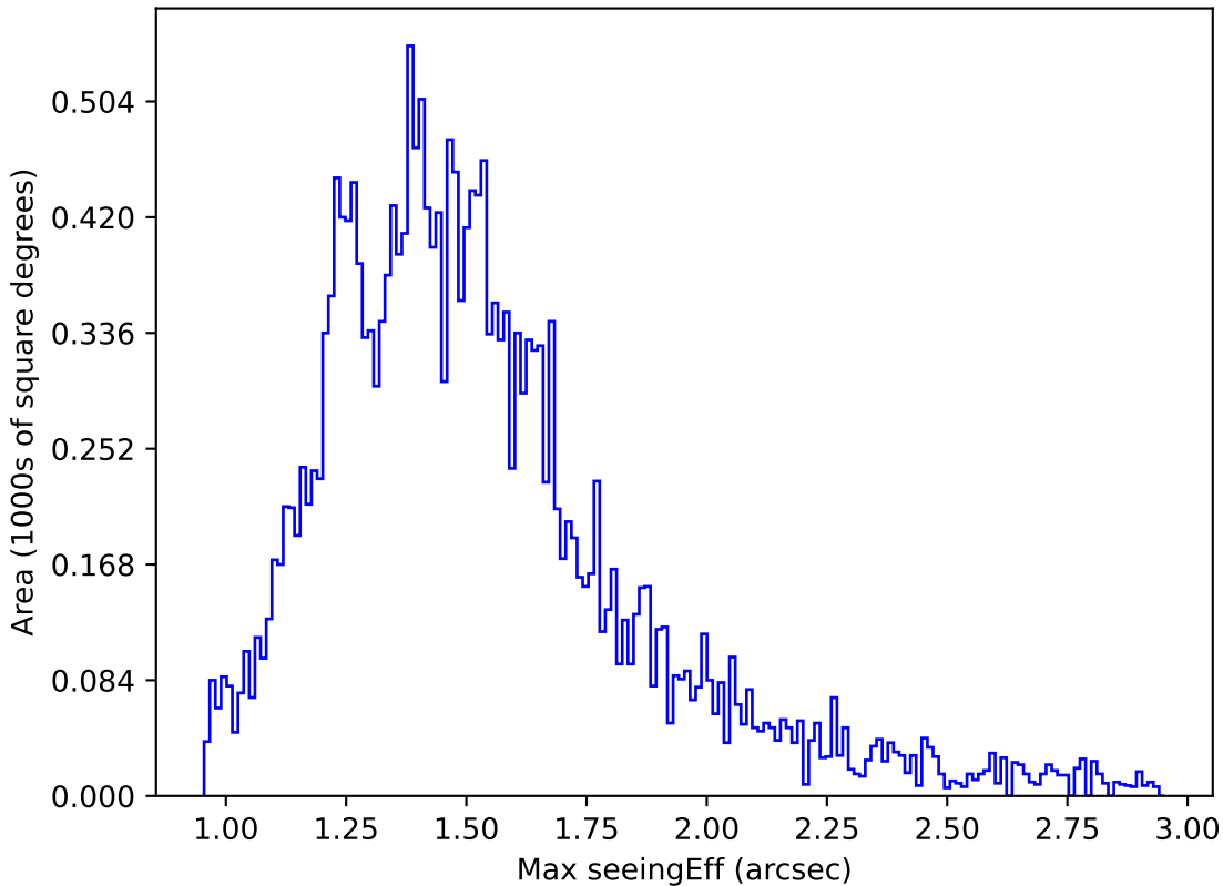
too_5_4v3.4_10yrs Yr 1 u band: Max seeingEff
