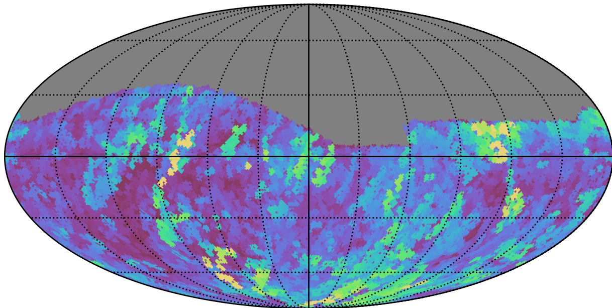
too_5_4v3.4_10yrs Yr 1 r band: Max seeingEff
