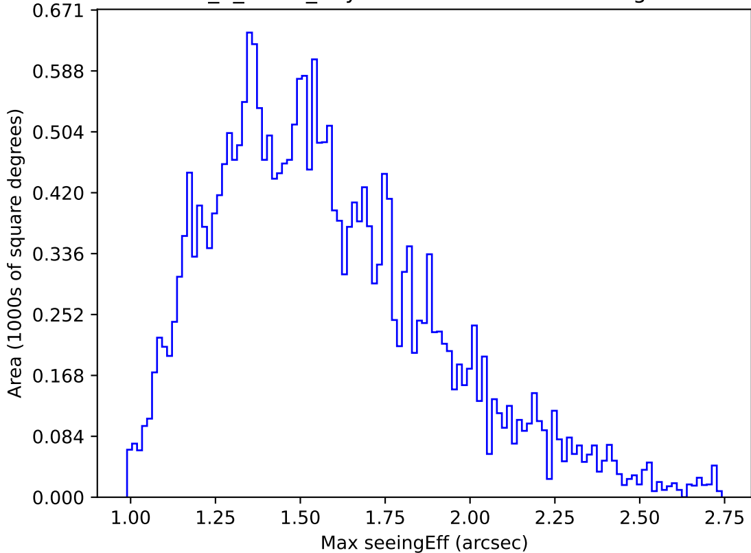
too_5_4v3.4_10yrs Yr 1 r band: Max seeingEff
