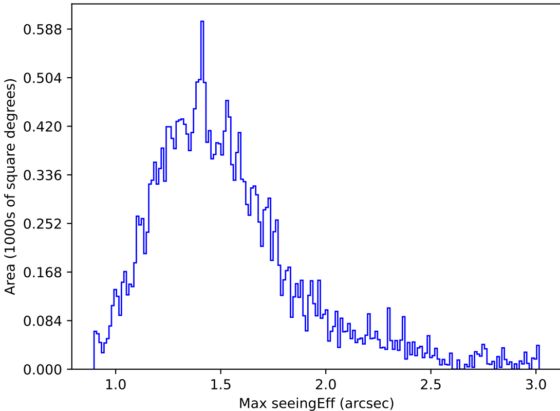
too_5_4v3.4_10yrs Yr 1 i band: Max seeingEff
