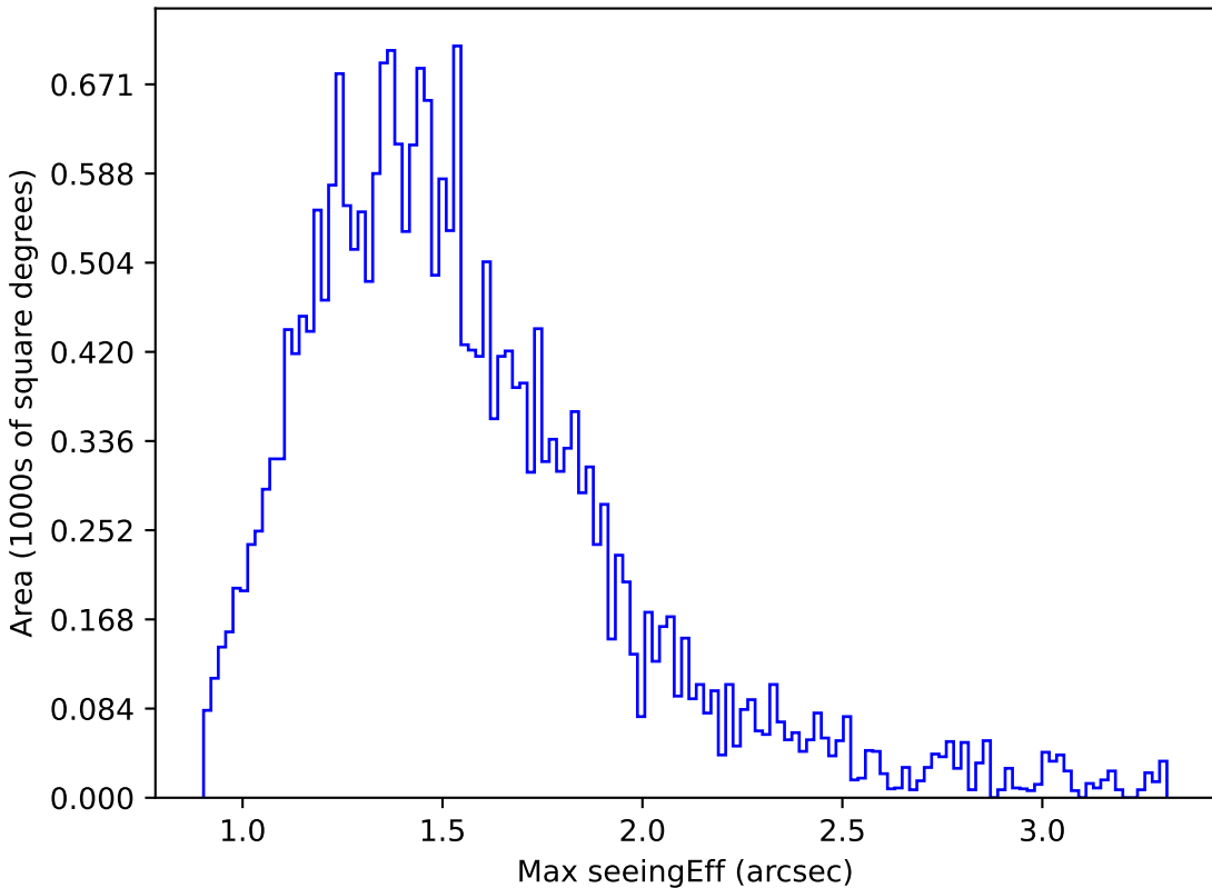
too_5_4v3.4_10yrs Yr 1 g band: Max seeingEff
