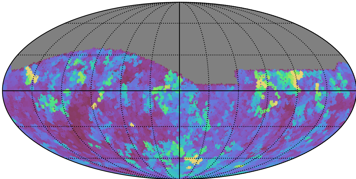
too_5_4v3.4_10yrs Yr 1 all bands: Max seeingEff
