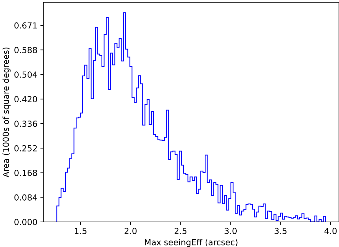
too_5_4v3.4_10yrs Yr 1 all bands: Max seeingEff
