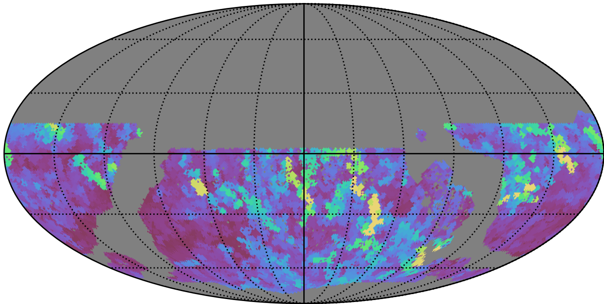
too_5_4v3.4_10yrs WFD z band: Max seeingEff
