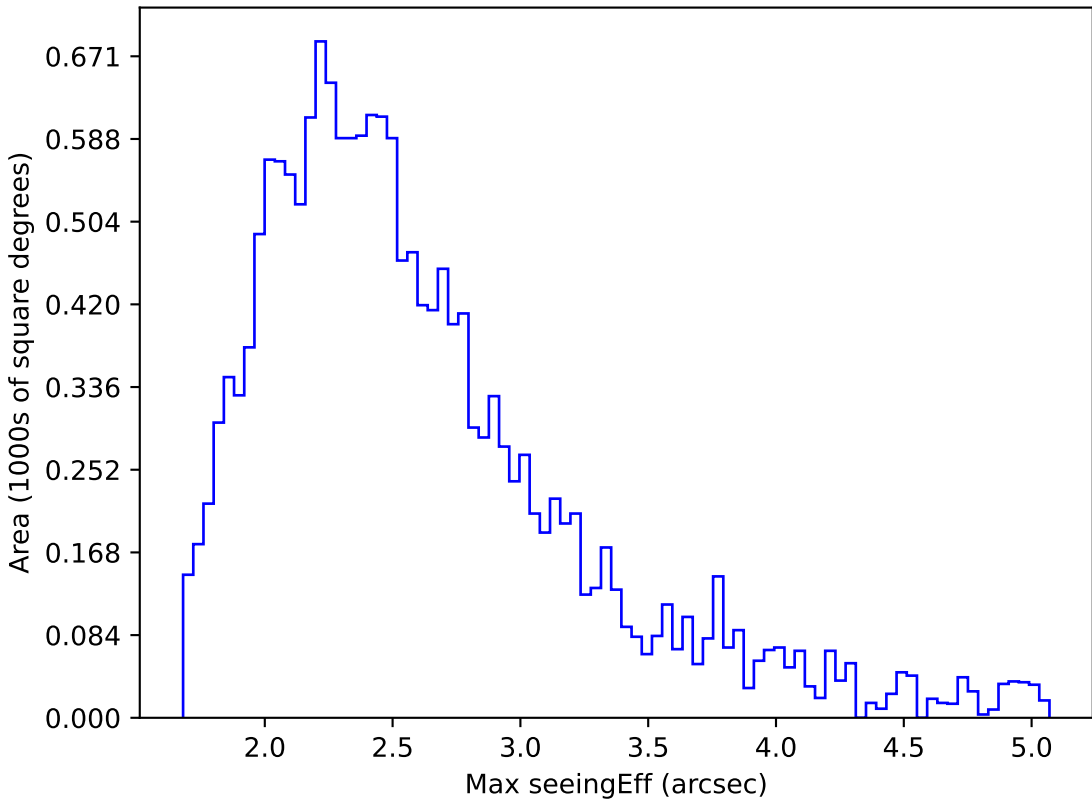
too_5_4v3.4_10yrs WFD z band: Max seeingEff
