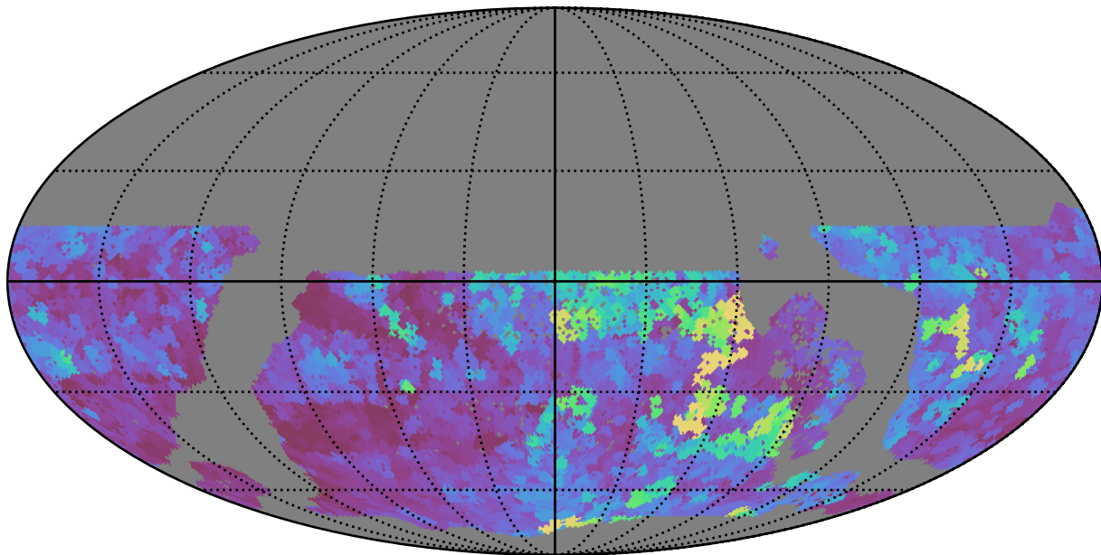
too_5_4v3.4_10yrs WFD y band: Max seeingEff
