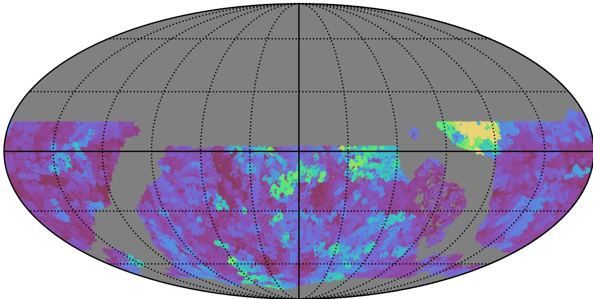
too_5_4v3.4_10yrs WFD u band: Max seeingEff
