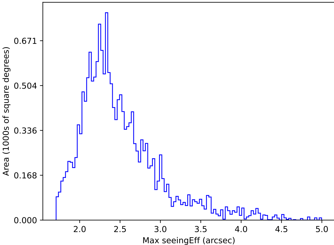
too_5_4v3.4_10yrs WFD u band: Max seeingEff
