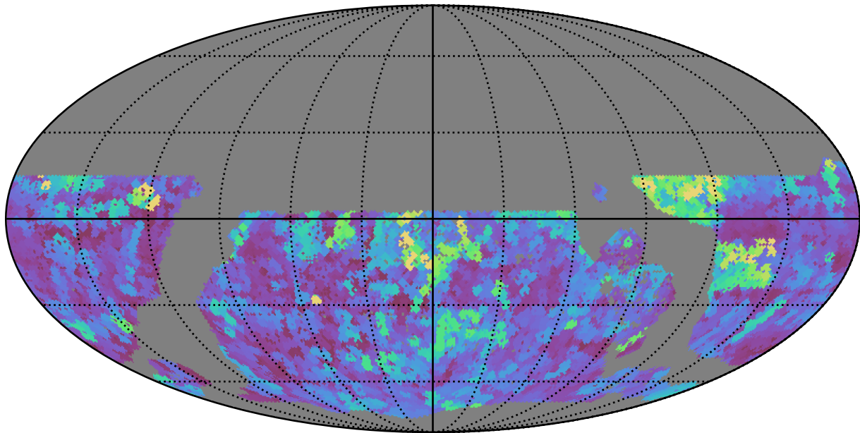
too_5_4v3.4_10yrs WFD r band: Max seeingEff
