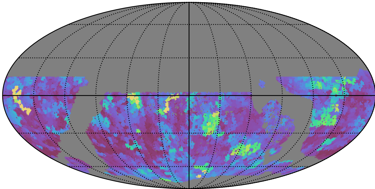
too_5_4v3.4_10yrs WFD i band: Max seeingEff
