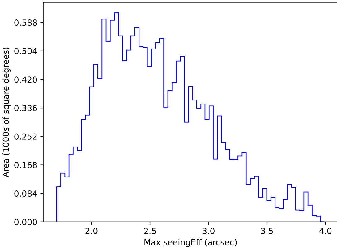
too_5_4v3.4_10yrs WFD g band: Max seeingEff
