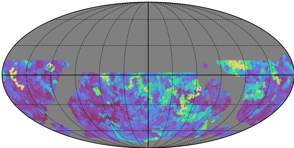
too_5_4v3.4_10yrs WFD all bands: Max seeingEff
