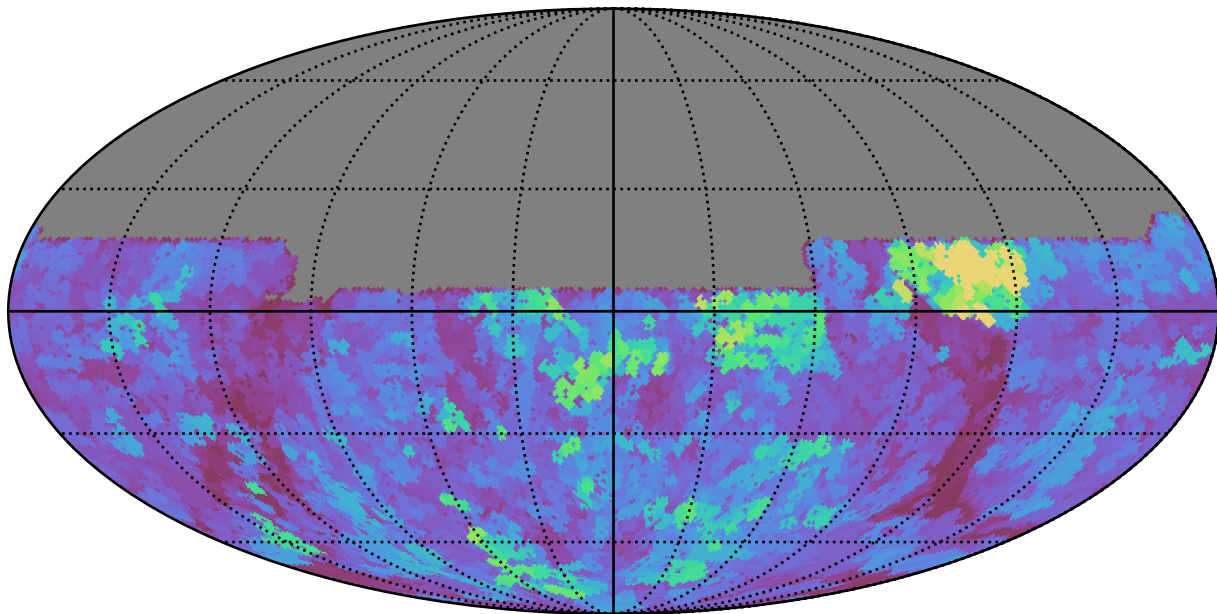
too_5_4v3.4_10yrs All sky u band: Max seeingEff
