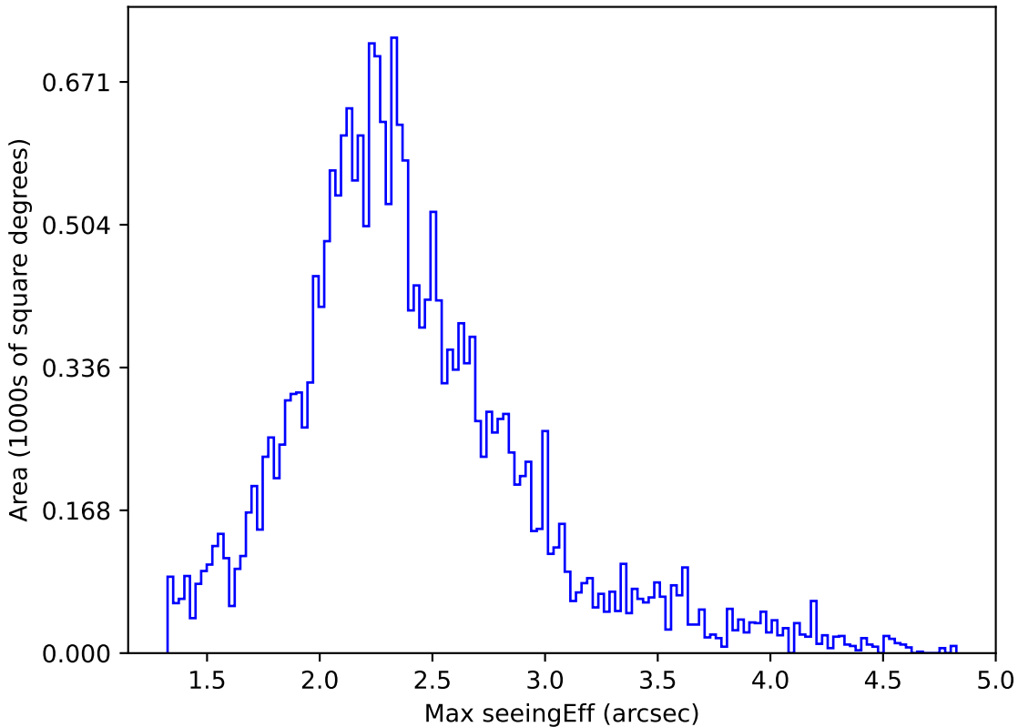
too_5_4v3.4_10yrs All sky u band: Max seeingEff
