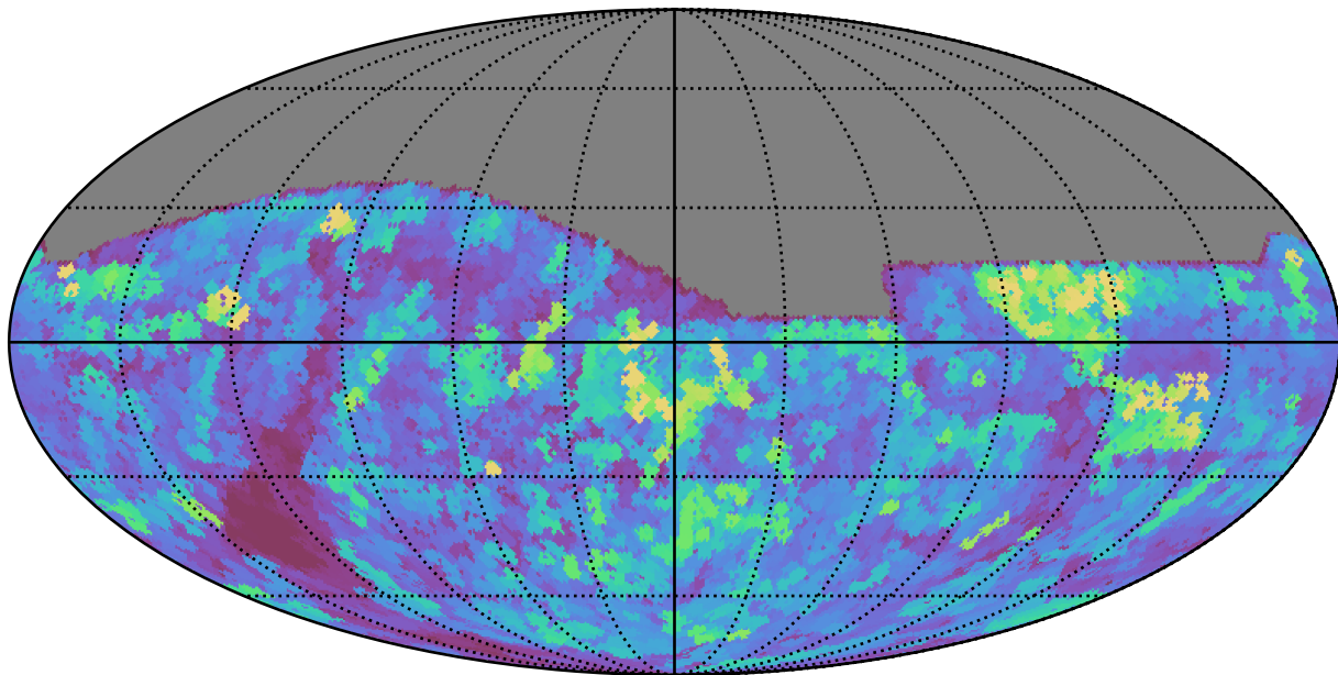
too_5_4v3.4_10yrs All sky r band: Max seeingEff
