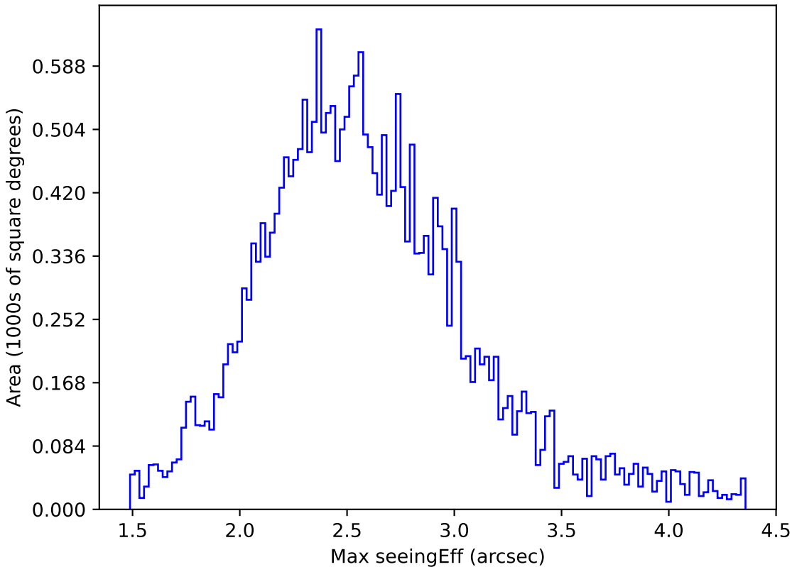
too_5_4v3.4_10yrs All sky r band: Max seeingEff
