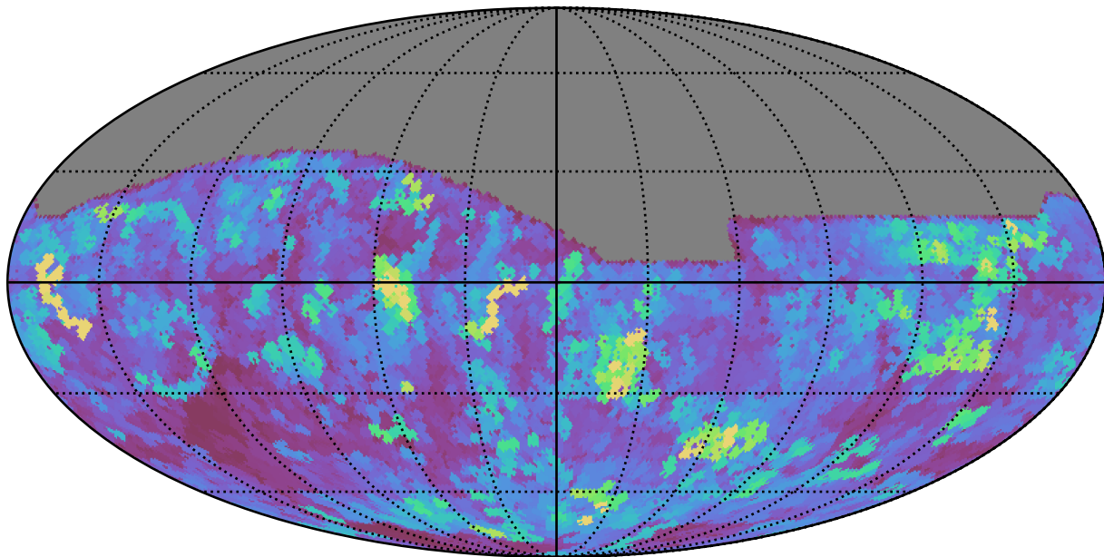
too_5_4v3.4_10yrs All sky i band: Max seeingEff
