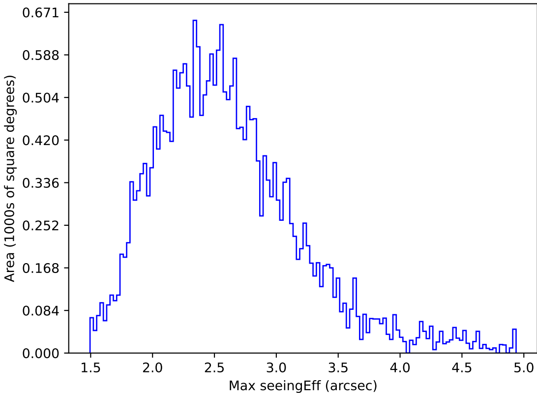
too_5_4v3.4_10yrs All sky i band: Max seeingEff
