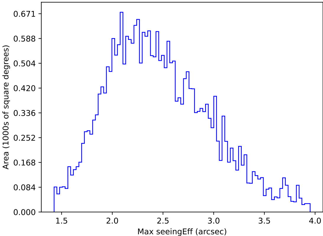
too_5_4v3.4_10yrs All sky g band: Max seeingEff
