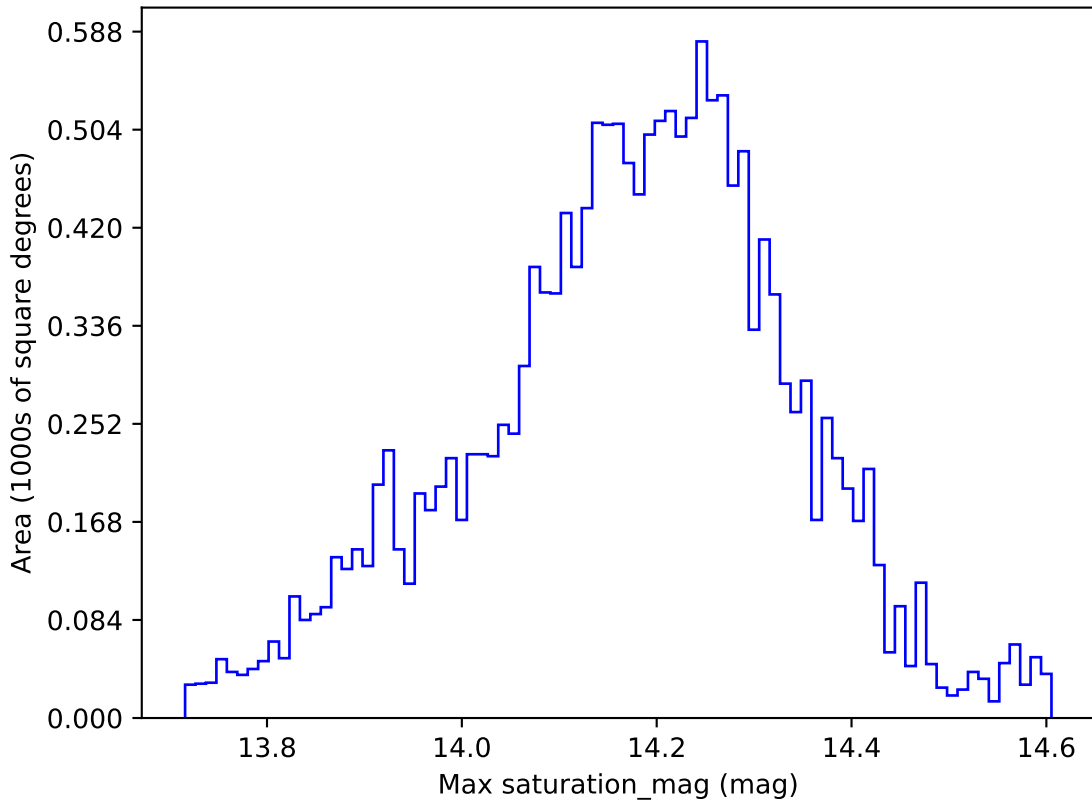
too_5_4v3.4_10yrs WFD y band: Max saturation_mag
