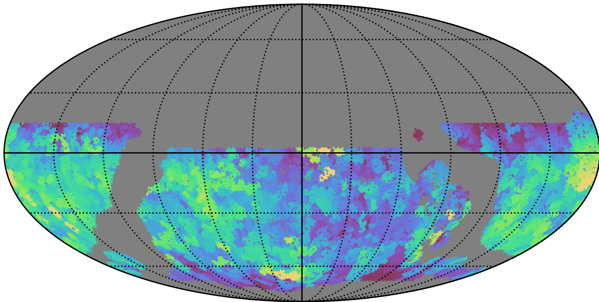
too_5_4v3.4_10yrs WFD u band: Max saturation_mag
