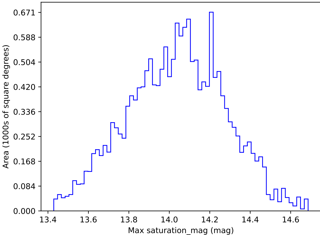
too_5_4v3.4_10yrs WFD u band: Max saturation_mag
