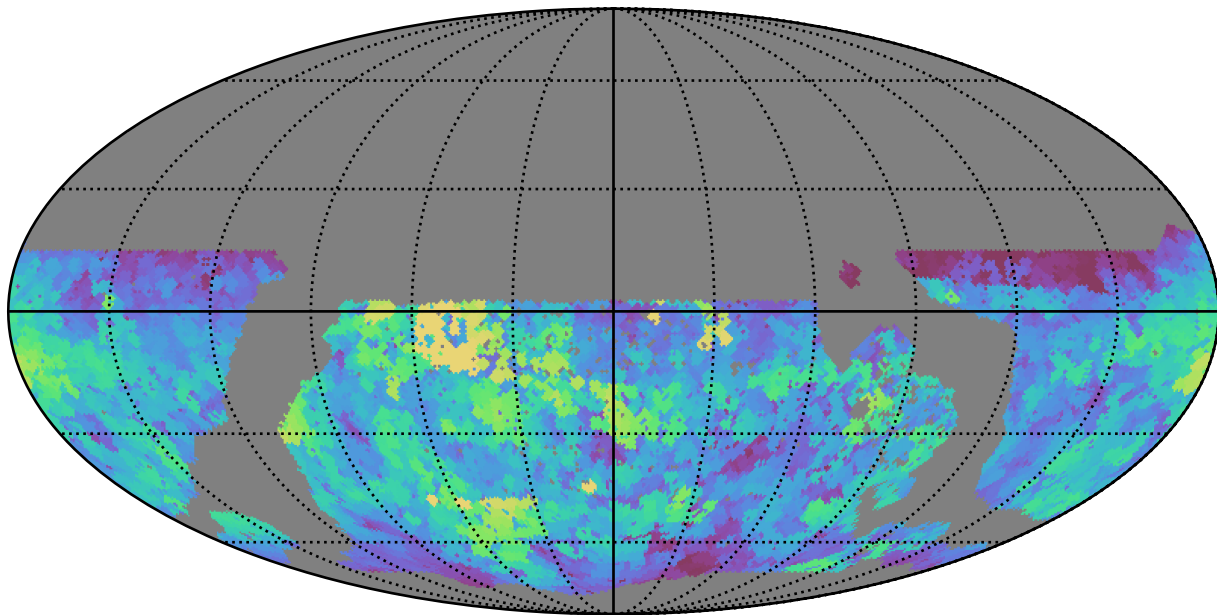
too_5_4v3.4_10yrs WFD g band: Max saturation_mag
