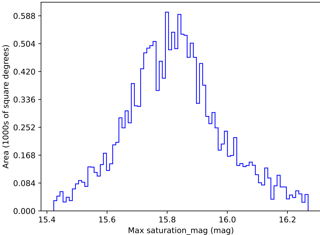
too_5_4v3.4_10yrs WFD all bands: Max saturation_mag
