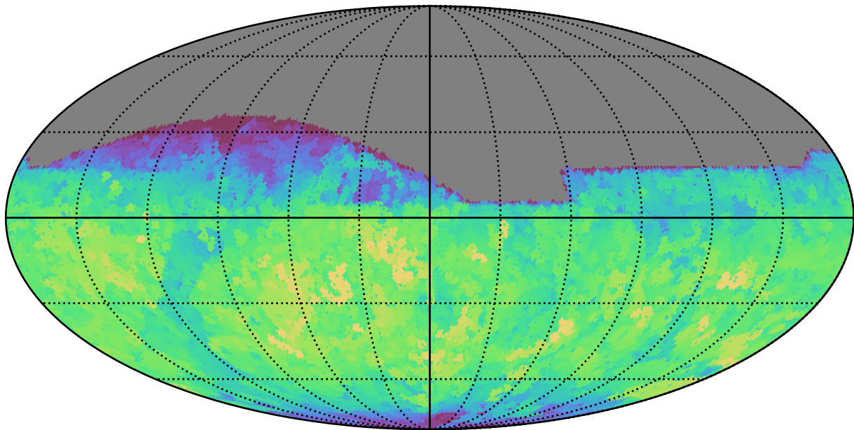
too_5_4v3.4_10yrs All sky z band: Max saturation_mag
