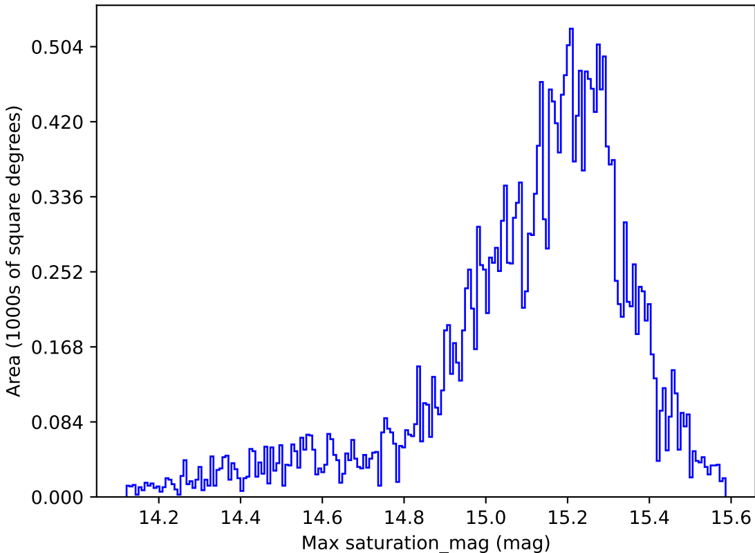
too_5_4v3.4_10yrs All sky z band: Max saturation_mag
