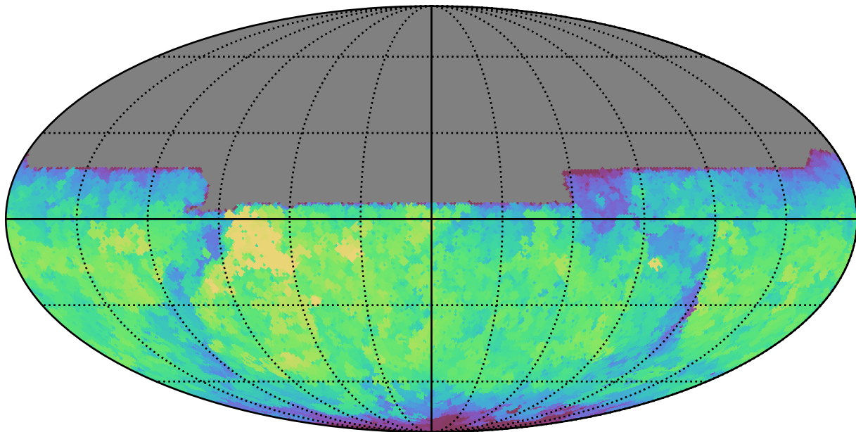
too_5_4v3.4_10yrs All sky y band: Max saturation_mag
