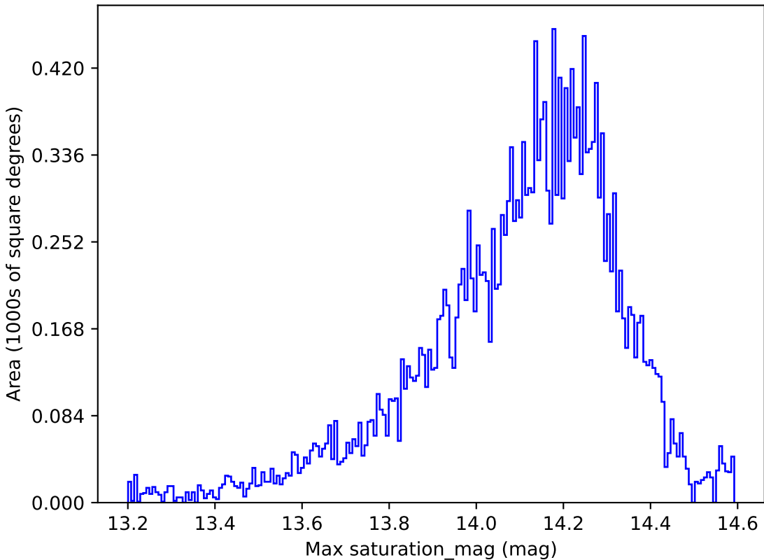
too_5_4v3.4_10yrs All sky y band: Max saturation_mag
